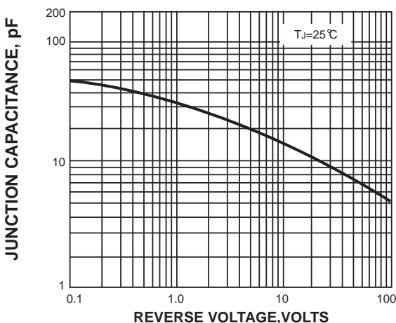
FIG. 5-TYPICAL JUNCTION CAPACITANCE
