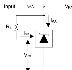
Test Circuit for I_{ref}
