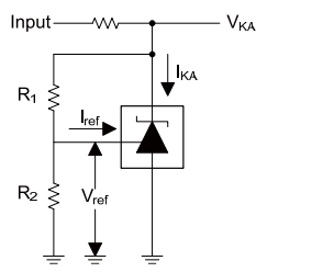
Test Circuit for V_{KA}=V_{ref}(1+R1/R2)+R1*I_{ref}
