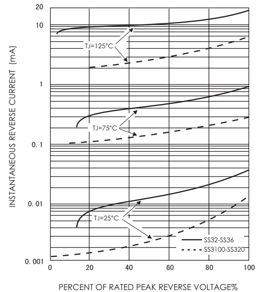
FIG.4-TYPICAL REVERSE CHARACTERISTICS
