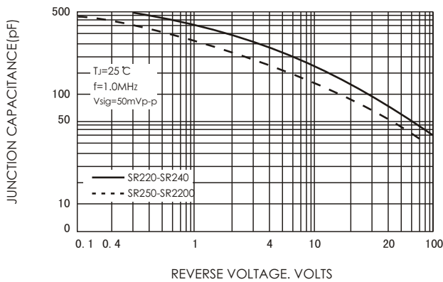
FIG.5-TYPICAL JUNCTION CAPACITANCE
