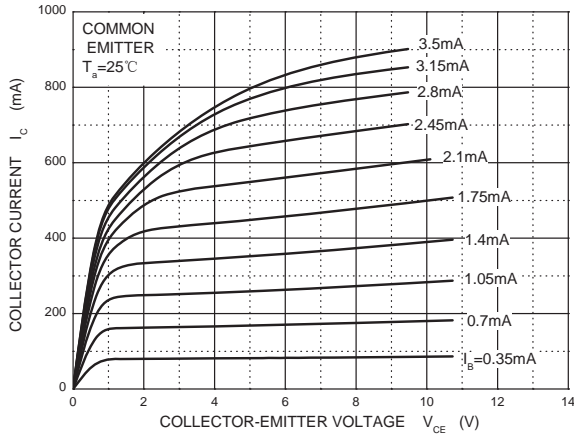
Static Characteristic
